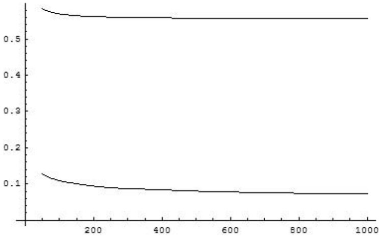
Fig. 2. Capacity of the bipolar network with N \in \{50, \dots, 1000\} neurons and Q = 4 , compared with the bound given by McEliece (lower graph)
