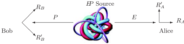
Fig. 2. Measuring entangled pairs |EP\rangle
