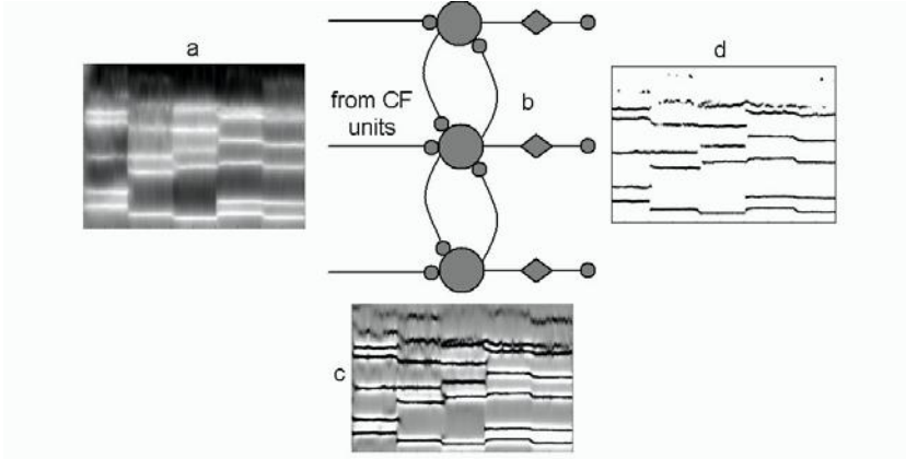
Fig. 7. Formant Detection for the utterance /aeiou/: The speech spectral density (a) is processed by columns of neurons implementing lateral inhibition (b), producing differentially expressed formant lines (c), which are transformed into narrow formant trajectories (d) after non-linear saturation
