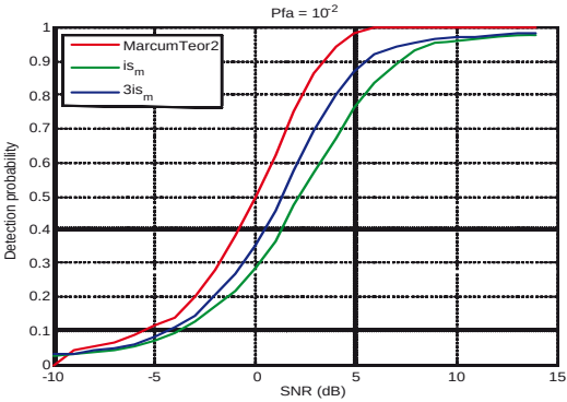
Fig. 5. Detection probability, P_{fa}=10^{-2} , threshold 0.2
