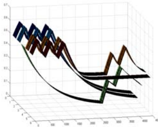
Fig. 6. Evolution of the shift of the activation function. During the first 1250 alpha and gamma neuron's shift is around 0.5. After injury the shift decreases so that the sigmoid moves leftwards. After treatment (iteration 3000) only the shift of the alpha and Ia neuron increase.
