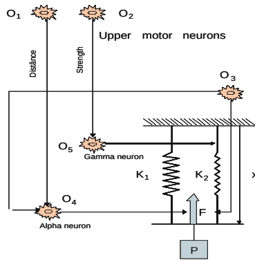
Fig. 1. Simplified scheme of the neural circuit involved in motor control. The muscle has been substituted by two springs representing extrafusal and intrafusal fibers. O_3 represents the output of the, so called, Ia neurons whose axons are coiled in intrafusal fibers.
