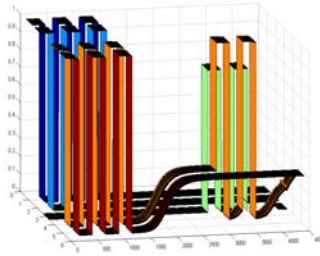
Fig. 5. The evolution of spasticity before and after injury is depicted in this figure. Vertical axis represent the output (firing probability) of the different neurons in the network. Ribbons from back to front represent outputs O_1 , O_2 , O_3 , O_4 and O_5 .
