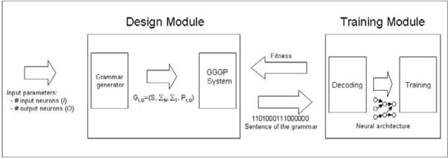
Fig. 3. Neuroevolution system
