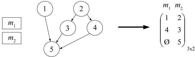
Fig. 1. Dependency graph associated with the set of tasks T = \{1, 2, 3, 4, 5\} together with an optimal scheduling grid for a two-processor scenario m_1 and m_2
