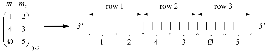
Fig. 2. Representation of a scheduling grid in a DNA strand by means of row concatenation. ( N = 3 and M = 2 ).
