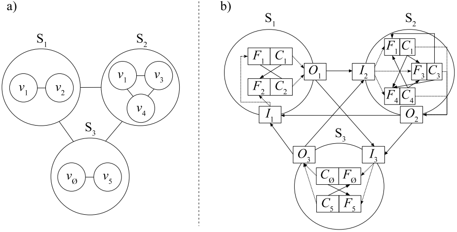
Fig. 3. a) Diagram of the two-layer system S associated with the example in Fig. 1. It is composed of three subsystems each with several nodes: S_1 = \{v_1, v_2\} , S_2 = \{v_1, v_3, v_4\} , S_3 = \{v_5, v_0\} . b) Design of the microfluidic device for the system S shown in Fig. 3 a). Each element v_j is composed of a filter chamber F_j and a concatenation chamber C_j . Additionally, all the subsystems S_i have an inlet chamber I_i and an outlet chamber O_i .
