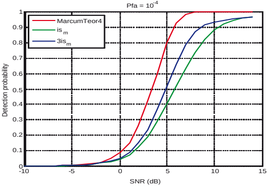
Fig. 7. Detection probability, P_{fa}=10^{-4} , threshold 0.2
